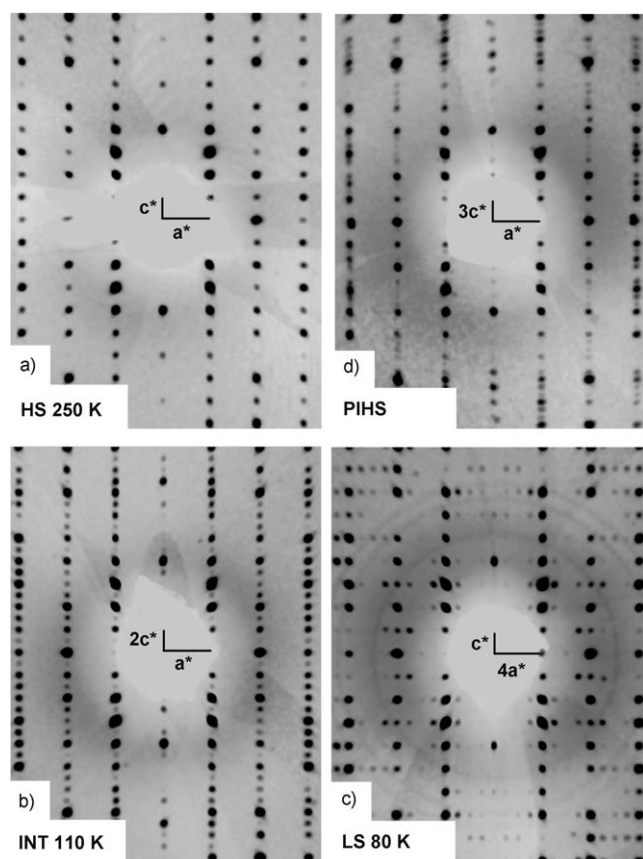
Figure 3. Reconstructed diffracted intensity in the a^*c^* reciprocal plane. With respect to the HS reciprocal lattice at 250 K, new peaks appear at l + 1/2 in the INT phase, at h + 1/4, + 1/2, + 3/4 in the LS phase, and at l + 1/3, + 2/3 in the PIHS phase.
